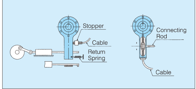
Structure of speed controlling section
